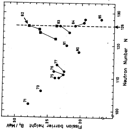
Fig. 3. Experimental data [2,7,9] on the fission barrier heights B_f of preactinide nuclei with Z and N close to the doubly magic nucleus ^{208}\text{Pb} ; the results of refs. [3,4,6] give a similar picture of B_f changes as a function of Z and N in this region.
