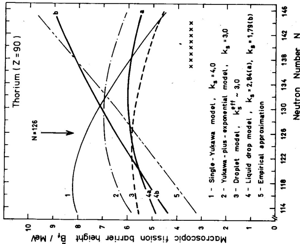
Fig. 2. Isospin dependence of the macroscopic fission barrier heights B_f for Th isotopes, calculated in terms of the LDM and its modifications (1 - the model of Krappe and Nix 86/ ; 2 - a modified version 87/ of the Krappe and Nix model; 3 - the DM of Myers 85/ ; 4a and 4b - the LDM using the parameters of Pauli and Ledergerber 40/ and of Myers and Swiatecki 20/ , respectively; 5 - an empirical approximation 88/ , B_f = 12.5 - 2.7(33.5 - Z^2/A)^{2/3} MeV, obtained by fitting an analytical expression to the results of extraction of shell corrections to ground-state nuclear masses from the experimental values of fission barrier heights). The Th isotopes for which there are experimental data on fission barriers are indicated by (x).
